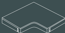
| AF 40/GetaCore® | one piece corner top L-form 1180 x 1180 x 600 x 39 mm
